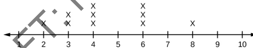
Figure 2.28 Maris' distribution is symmetrically shaped.
