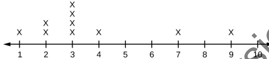
Figure 2.26 Terry's distribution has a right (positive) skew.
